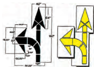
S-5015 D/M Arrow Combo Kit, 3 Pc. Highway/Intersection 13'-4" O.A.L. to Texas D.O.T. Spec. (Details vary per state)
